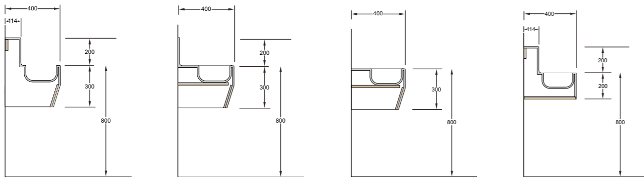
DfE1 Thermo Profile Thermoformed trough with wall mounted taps. A choice of underframe or brackets. DfE2 Thermo Profile Thermoformed trough with deck mounted taps. A choice of underframe or brackets. DfE3 Thermo Profile Thermoformed trough with deck mounted taps. A choice of underframe or brackets. DfE4 Thermo Profile Thermoformed trough with wall mounted taps. A choice of brackets or underframe.
