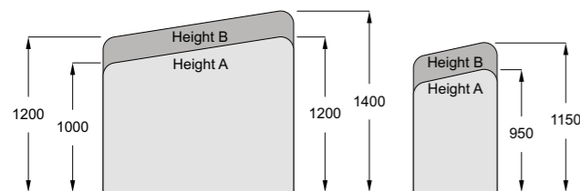
Door and partition height options
