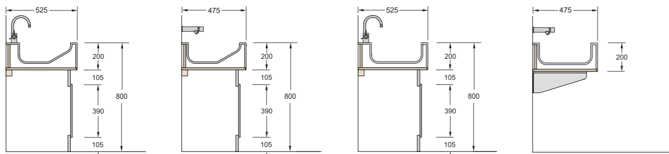
WT1 Thermo Profile Thermoformed trough with deck mounted taps. A choice of underframe or brackets. WT2 Thermo Profile Thermoformed trough with wall mounted taps. A choice of underframe or brackets. WT3 Thermo Profile Thermoformed trough with deck mounted taps. A choice of underframe or brackets. WT4 Thermo Profile Thermoformed trough with wall mounted taps. A choice of brackets or underframe.
