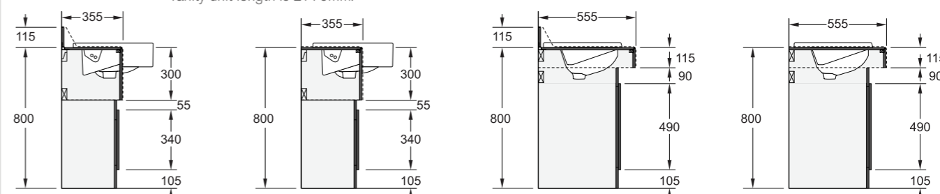
CV1 Profile Semi-recessed basin with upstand. CV2 Profile Semi-recessed basin without upstand. CV3 Profile Fully inset basin with upstand. CV4 Profile Fully inset basin without upstand.
