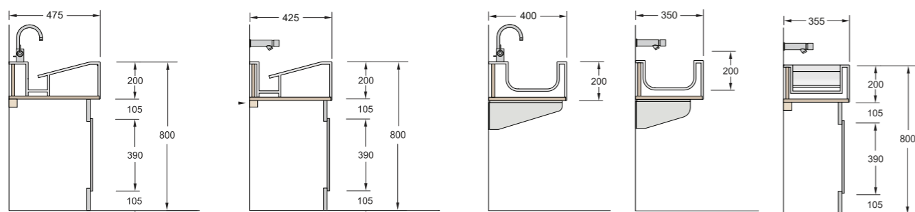
WT5 Profile Concealed waste trough with deck mounted taps. A choice of underframe or brackets. WT6 Profile Concealed waste trough with wall mounted taps. A choice of underframe or brackets. WT3 Thermo Slim Profile Slim thermoformed trough with deck mounted taps. A choice of brackets or underframe. WT4 Thermo Slim Profile Slim thermoformed trough with wall mounted taps. A choice of brackets or underframe. MyPod Profile Slim concealed waste trough with wall mounted taps. A choice of underframe or brackets.
