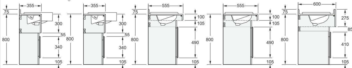
K1 Profile Semi-recessed basin with upstand. K2 Profile Semi-recessed basin without upstand. K3 Profile Fully inset basin with upstand. K4 Profile Fully inset basin without upstand. Baby Change Profile Fully inset basin with upstand.
