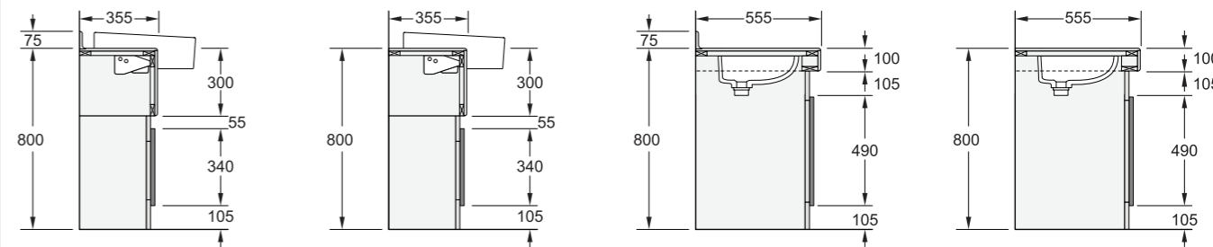
H1 Profile Semi-recessed basin with upstand. H2 Profile Semi-recessed basin without upstand. H3 Profile Fully inset basin with upstand. H4 Profile Fully inset basin without upstand.
